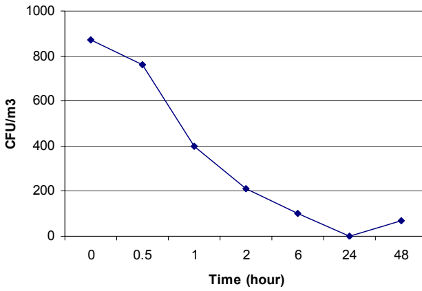
Fig. 5. Reduction in concentration of microorganisms in naturally contaminated air by two “TREE” air purifiers in an 83 \text{ m}^3 hospital room with door and windows closed and presence of one person.
